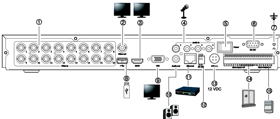
Figure 1: TVR 15HD/TVR 1516DHD back panel connections (16-channel models shown)
