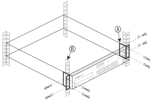
Figure 2: Rack-mount installation
