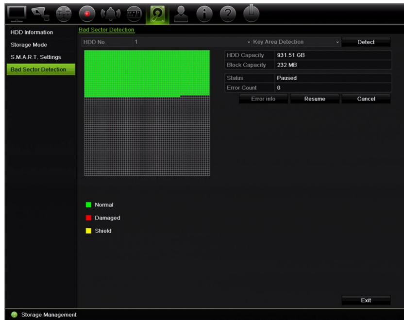
Figure 29: Bad sector detection window
